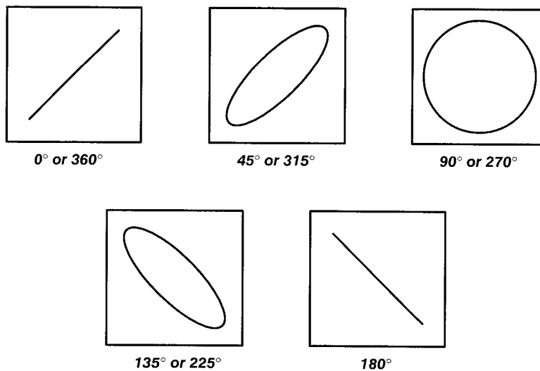
Figure 3-21: X-Y Phase Relationships
