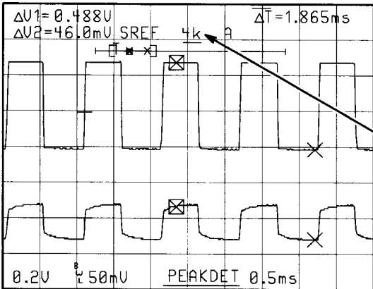
4K Two-Channel Acquisition Saved in Memory Location 4K.
