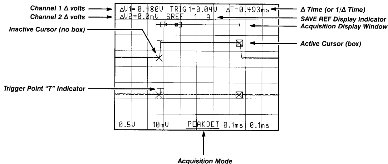
Figure 2-5: Digital (STORE) Mode Display
