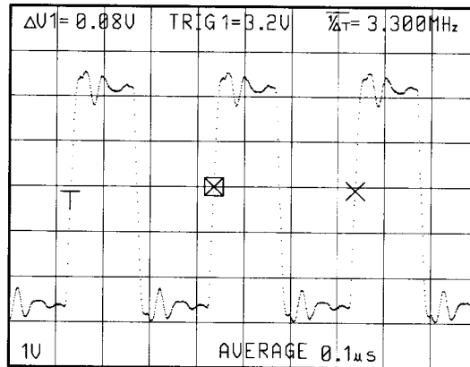
Figure 3-36: Cursor Frequency Measurement
