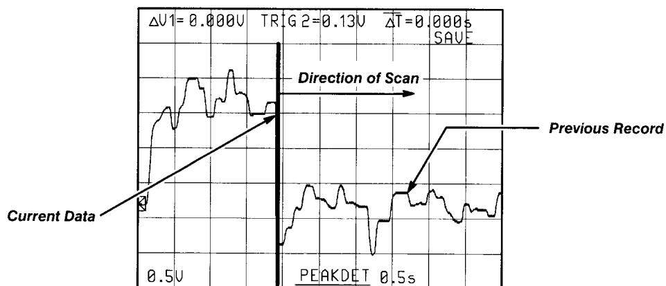
Figure 3-6: Scan Mode
