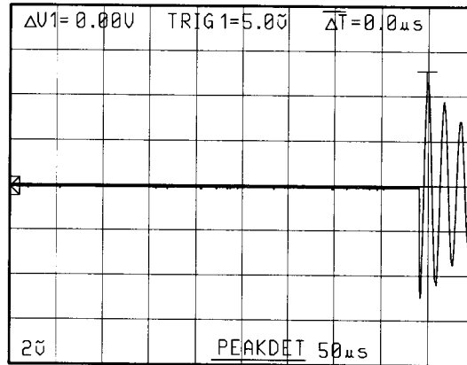
Figure 3-15: Pretrigger Acquisition
