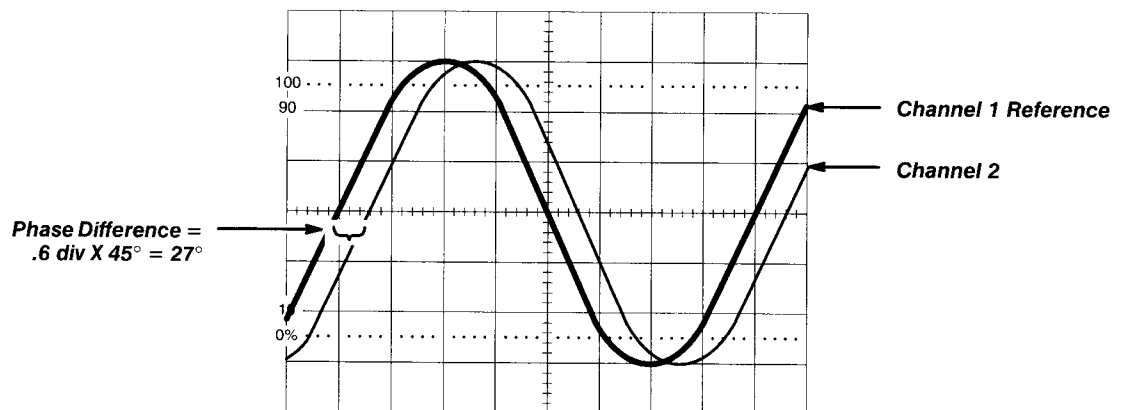
Figure 3-39: Measuring Phase Difference
