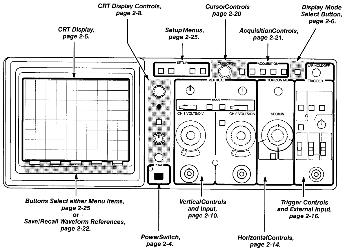
Figure 2-1: Front Panel Control Sections
