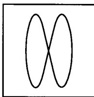
Figure 3-22: X-Y Frequency Relationships
