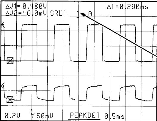
1K Two-Channel Acquisition Saved in Memory Location 1.
