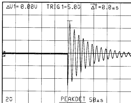
Figure 3-16: Midtrigger Acquisition
